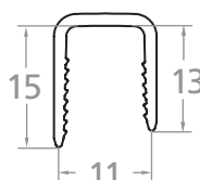
SE-111513 SPEED 11x15x13mm
