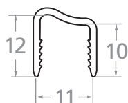
SE-111210A SPEEDARC 11x12x10mm
