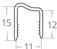
SE-111512A SPEEDARC 11x15x12mm
